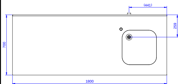
Shora
